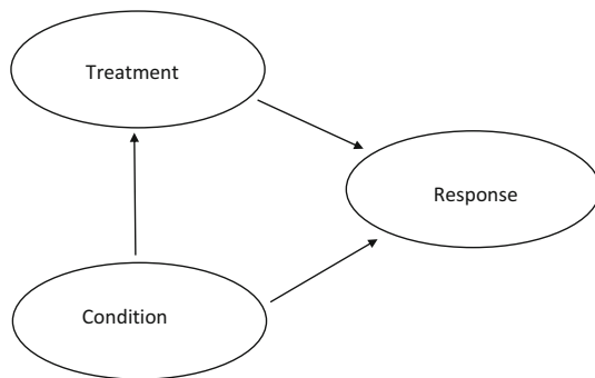
Fig. 6.6 Causal structure where a conditional analysis reveals the correct effect
