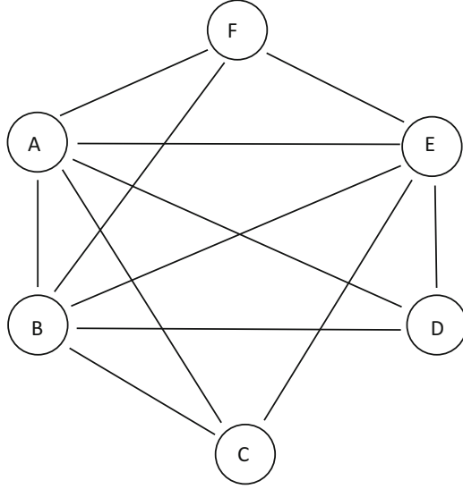
Fig. 2.5 The complement of this graph has one clique: CDF
