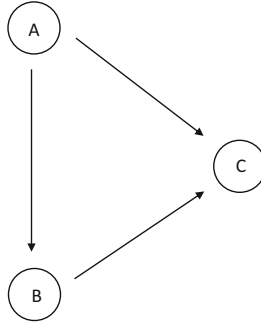
Fig. 4.1 A DAG, where conditional independence does not necessarily imply d-separation
