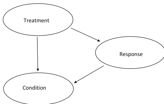
Fig. 6.4 Causal structure where a marginal analysis reveals the correct effect
