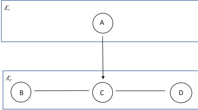
Fig. 10.2 A chain graph where the Type II model is not smooth
