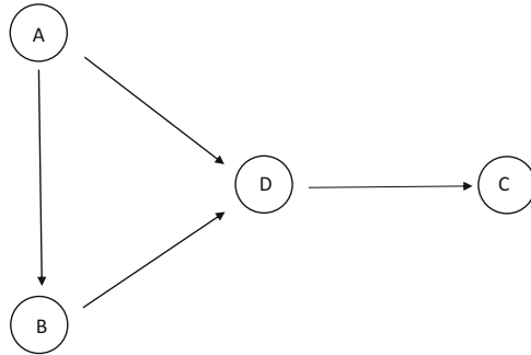
Fig. 3.3 DAG, according to which a distribution is directed pairwise Markov but not directed local Markov
