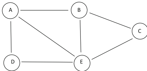
Fig. 3.10 The triangularization of the graph in Fig. 3.9
