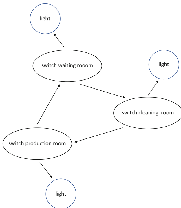
Fig. 6.7 An example of cyclic causality
