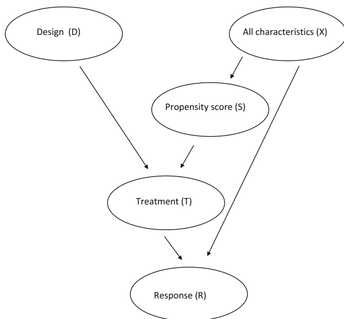
Fig. 6.3 DAG representation of the propensity score method
