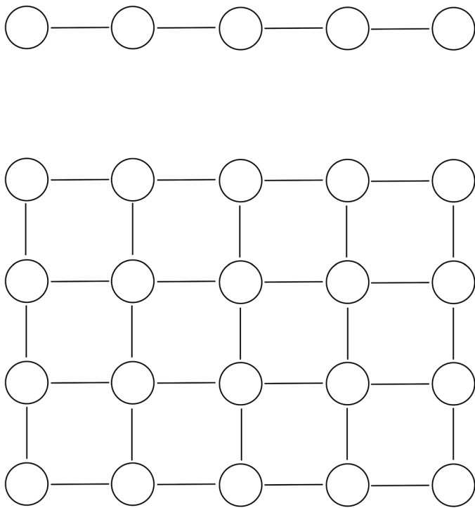
Fig. 2.3 The top graph is a Markov chain, and the bottom graph is an Ising model
