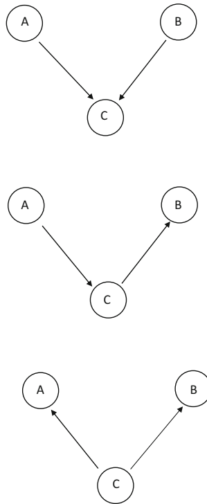
Fig. 3.4 Collider, intermediate (or chain), and fork configurations
