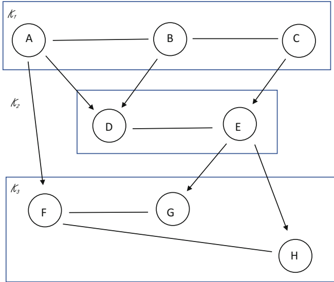
Fig. 3.11 A chain graph
