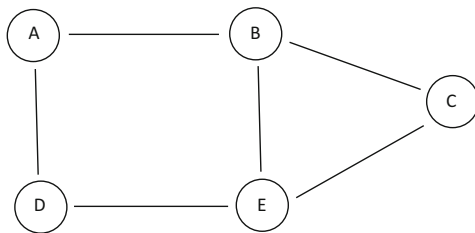
Fig. 3.9 The undirected moralization of the graph in Fig. 3.8
