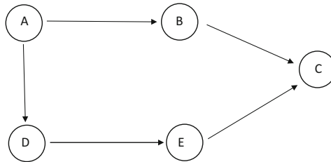
Fig. 3.8 Another DAG model of an expert system
