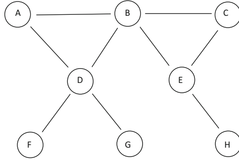
Fig. 3.6 Undirected moralization of the DAG in Fig. 3.5
