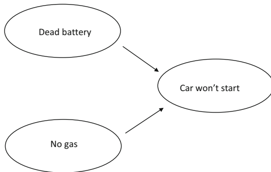
Fig. 6.1 A simplified causal structure described with a DAG—roadside assistance
