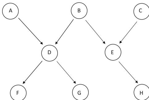
Fig. 3.5 A DAG model as an expert system. A, B, C are hard-to-test physiological functions of the human body; D, E are not easily observable medical conditions; and F, G, H are obvious symptoms
