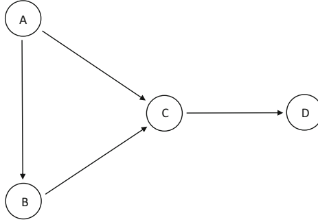
Fig. 5.1 The DAG for an illustration of IPCM
