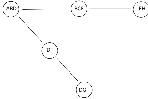
Fig. 3.7 A junction tree on the cliques of the undirected moralization of the DAG in Fig. 3.5
