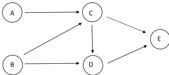
Fig. 10.1 A DAG, for which the marginal log-linear parameterizations are worked out
