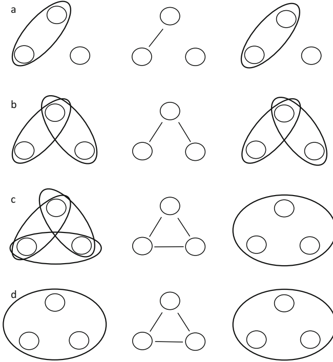
Fig. 2.1 Hypergraphs a , b , and d , are graphical, c is not. The figure shows hypergraphs with their respective 2-sections next to them and the clique hypergraphs obtained
