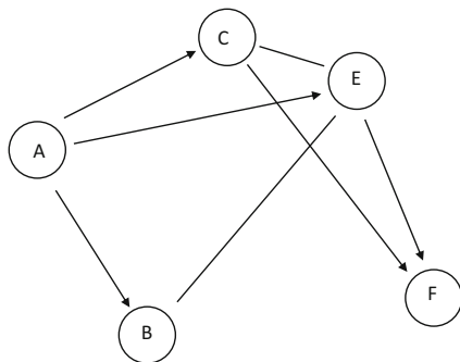
Fig. 3.2 The moralization (without the removal of direction) of the smallest ancestral subgraph containing \{A, B, C, E, F\} from the DAG in Fig. 3.1
