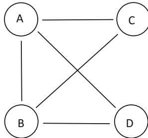
Fig. 2.4 A graph according to which the distribution in Table 2.1 is Markov but not faithful to it and is not Markov according to any of its subgraphs
