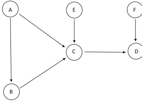
Fig. 5.2 The DAG of another illustration of IPCM
