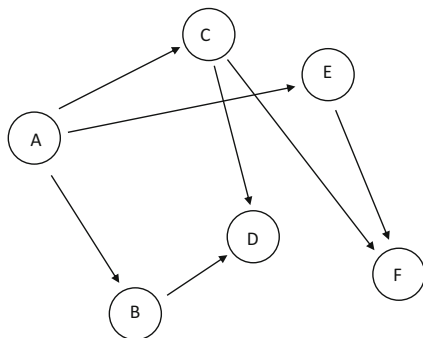
Fig. 3.1 Does the global Markov property imply that (A, B) \perp (E, F) | C ?
