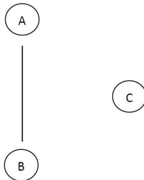
Fig. 2.2 If A = B = C , the pairwise Markov property for this graph holds, but the local does not
