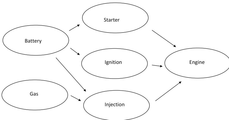
Fig. 6.2 A more complete causal structure—mechanic in the garage
