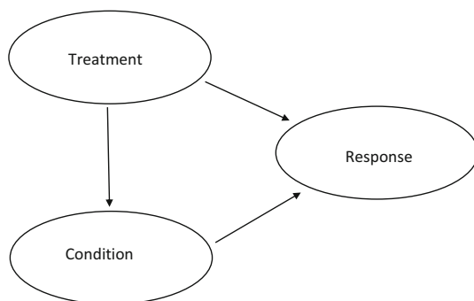
Fig. 6.5 Another causal structure where a marginal analysis reveals the correct effect
